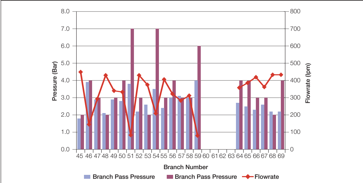
Figure 7: Recorded branch pressure, corresponding branch pass pressure and flowrate when supplied through 69m of 51mm hose at 4 bars pump pressure
