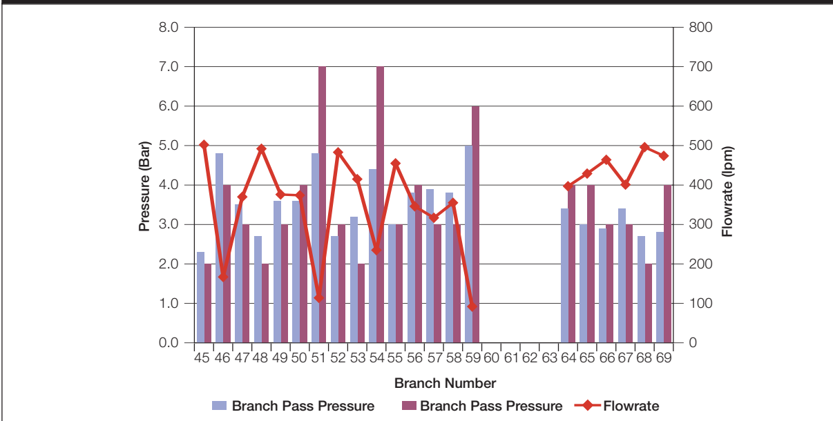
Figure 8: Recorded branch pressure, corresponding branch pass pressure and flowrate when supplied through 69m of 51mm hose at 5 bars pump pressure
